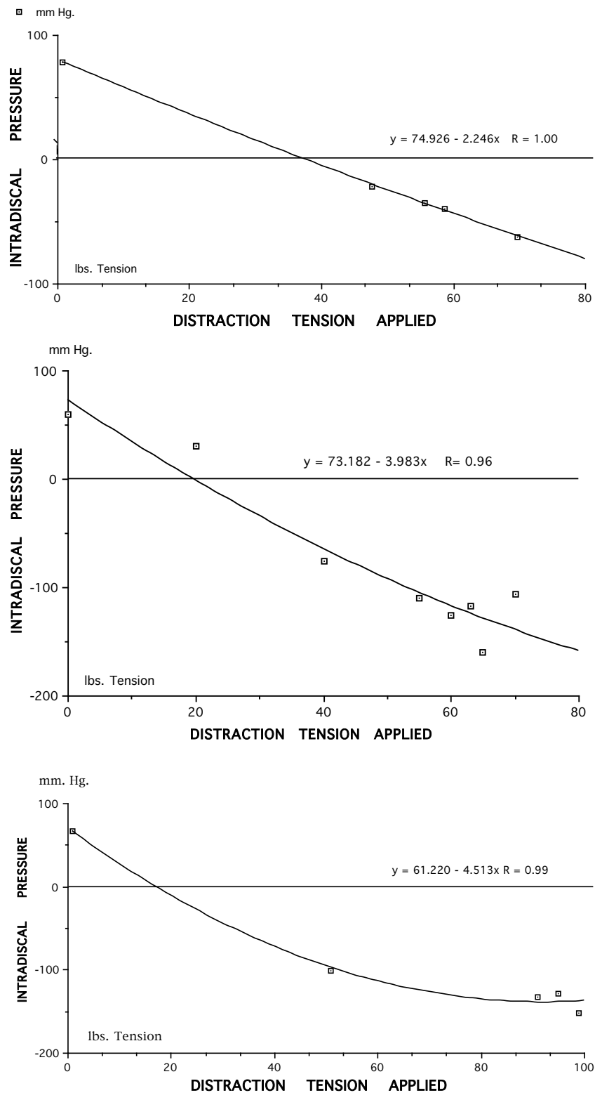
FIG. 2. Graphs showing the intradiscal pressures recorded in the L4-5 nucleus pulposus of three patients ( Case 3, upper; Case 4, center, and Case 5, lower) with a herniated disc at this level . Pressure is plotted against distraction tension consistent with the range of tension recommended as the therapeutic protocol for the equipment used in this study
